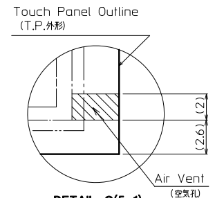
DETAIL C (5:1)
